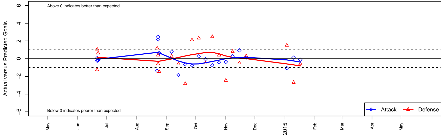
Seattle United W Blue B00 Dots are actual minus expected GF (blue circles) and GA (red triangles). Blue line is smoothed change in attack strength. Red is smoothed change in defense strength.
